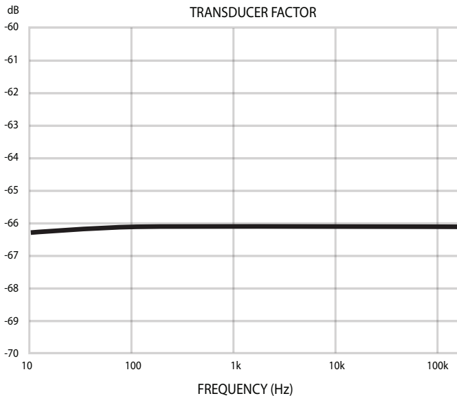
FLAT FREQUENCY RESPONSE
